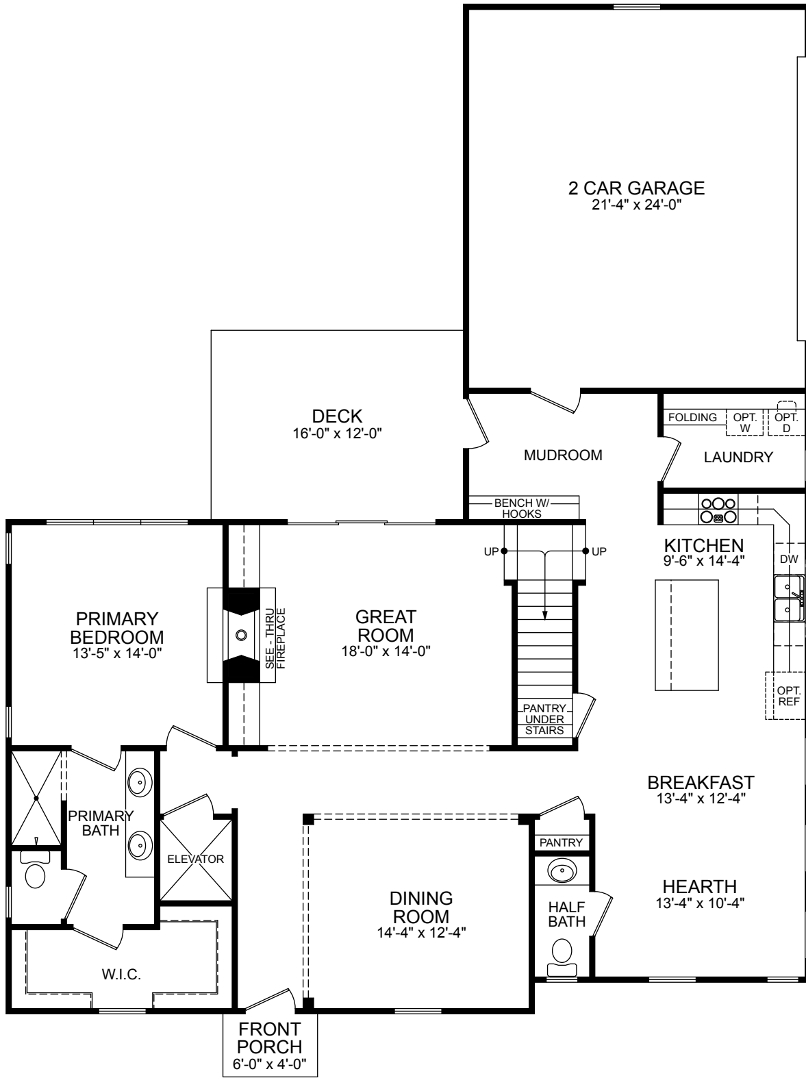
FIRST FLOOR
