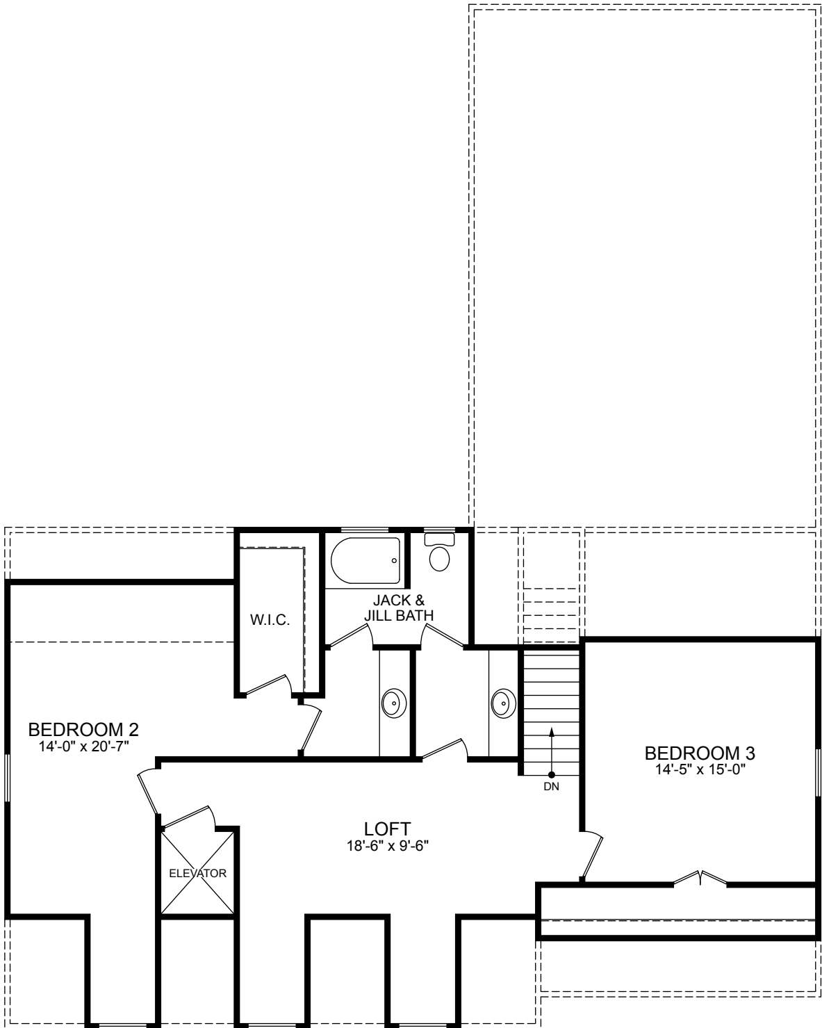
SECOND FLOOR
