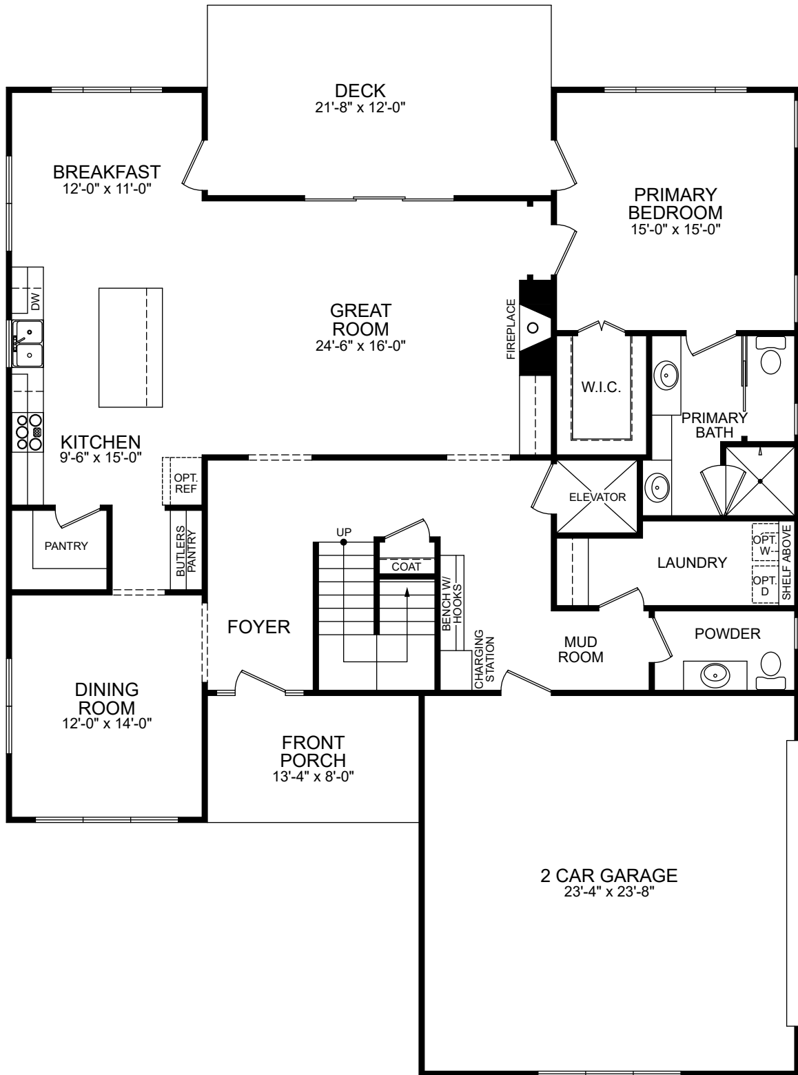
FIRST FLOOR
